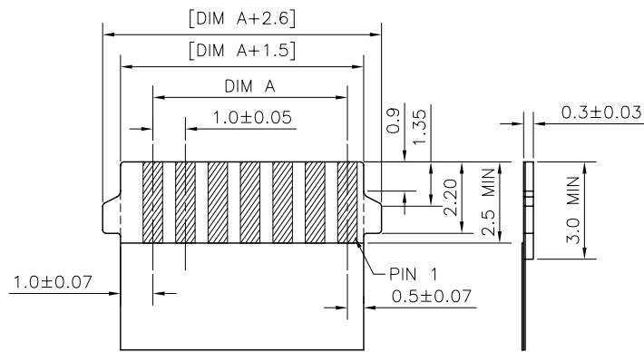
RECOMMENDED FPC/FPC DIMENSIONS GENERAL TOLERANCE ±0.1
